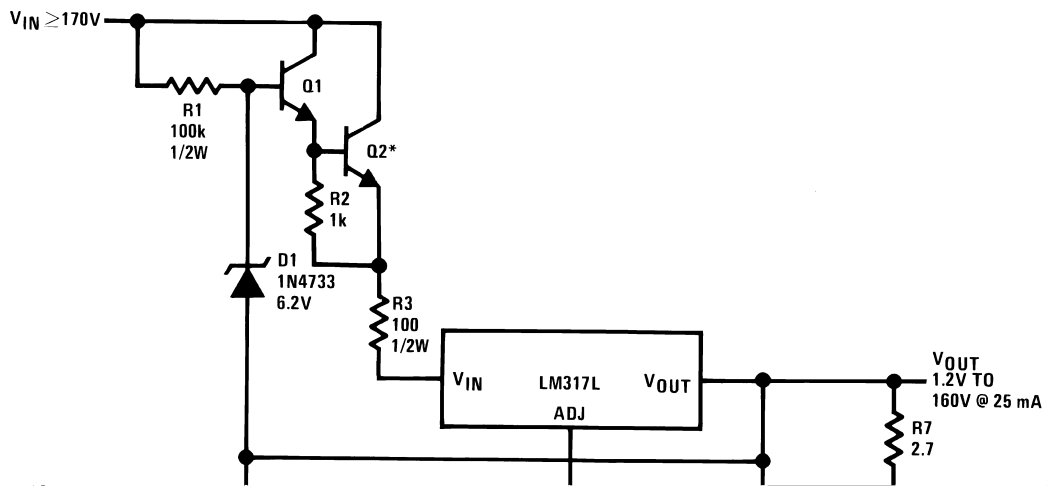
Basic High Voltage Regulator
